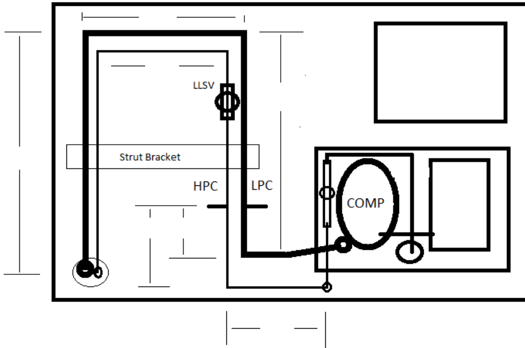
Skills PipingDiagram 1 2025
