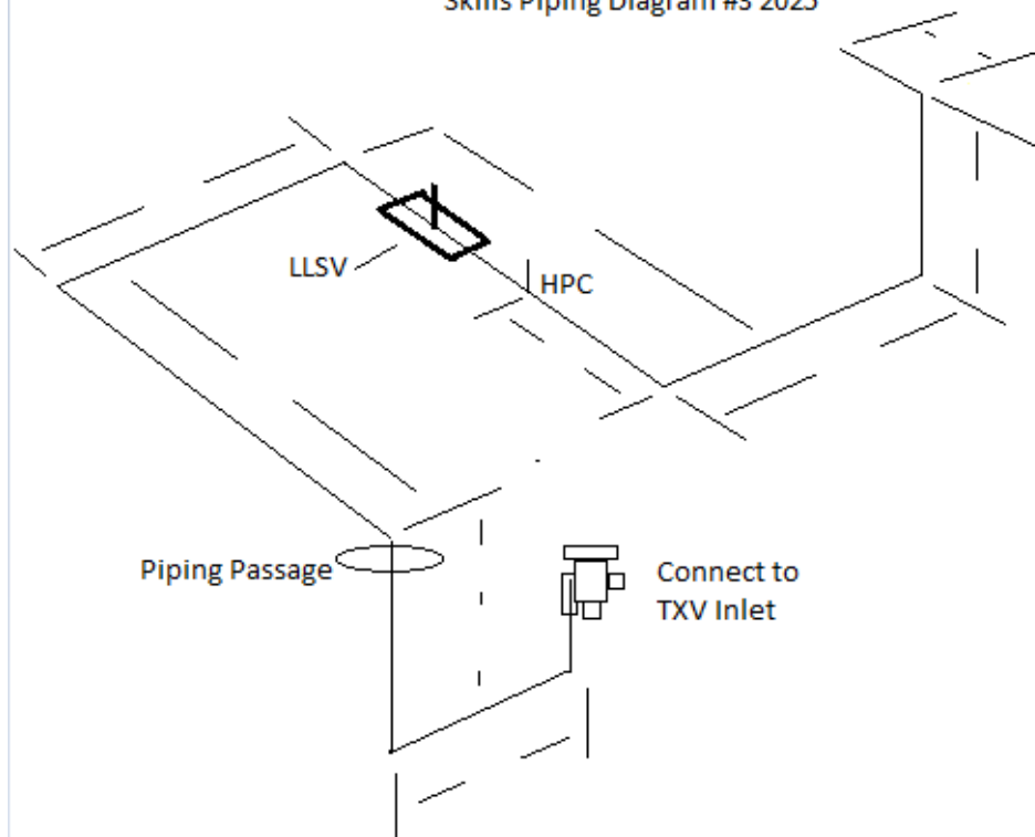
Skills Piping Diagram #3 2025
