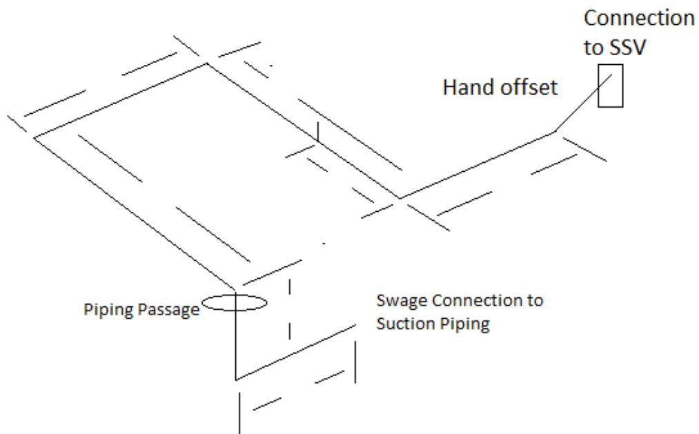
Skills Piping Diagram #3 2025
