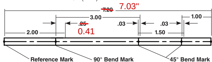
A – Unbent Tube with Markings
